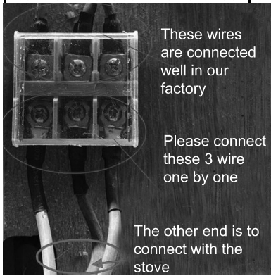
3-wires cable
